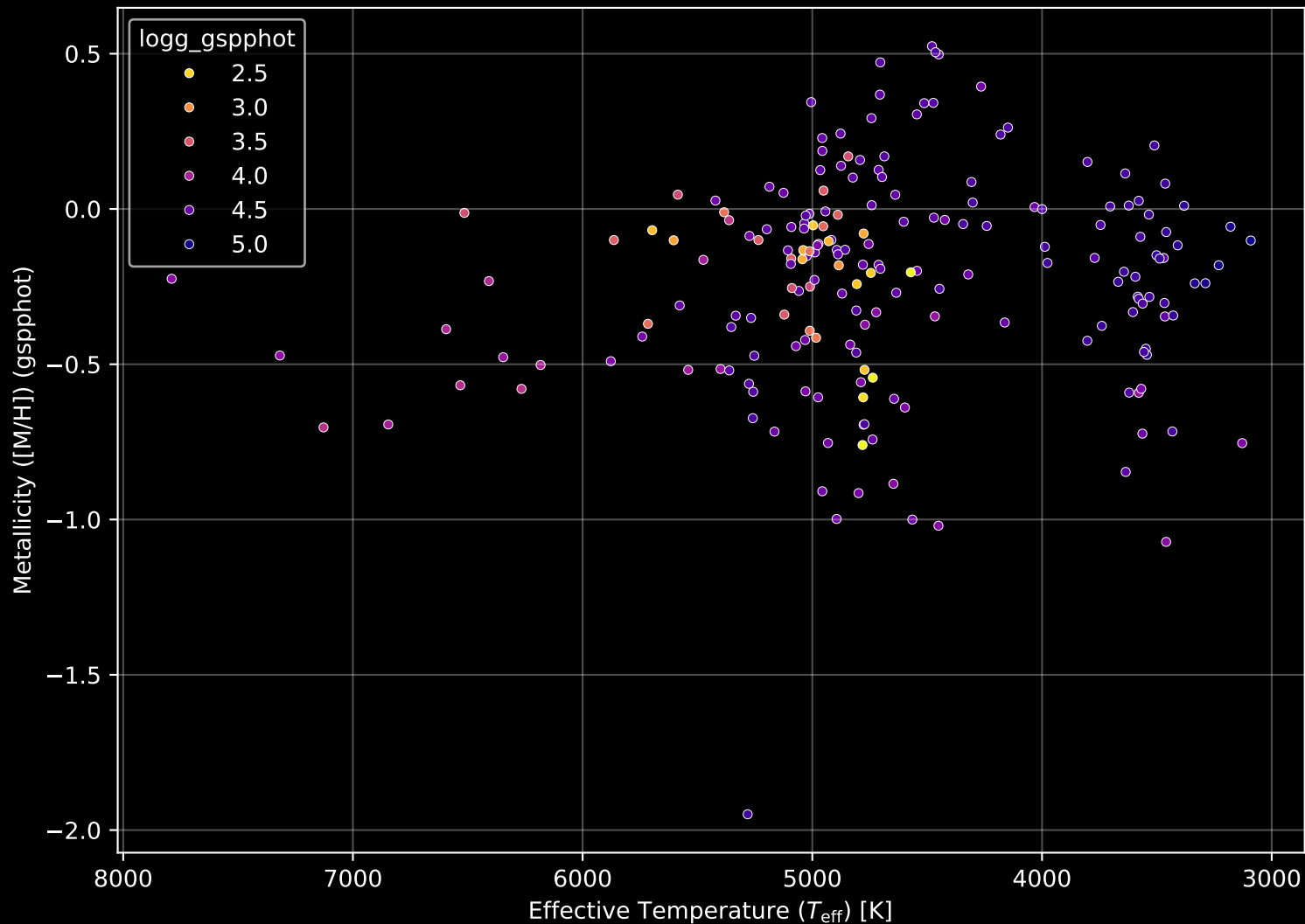
APOGEE DR17 Field: [K2_C8_129-62_btx] Stellar Population Parameters (n= 198)
