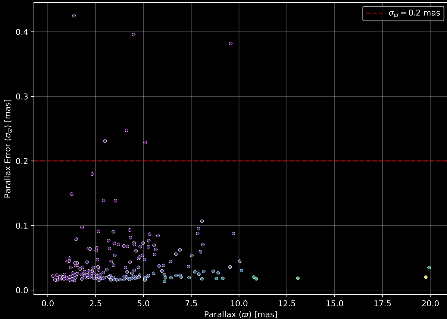
APOGEE DR17 Field: [K2_C8_129-62_btx] Parallax Quality (n= 198)
