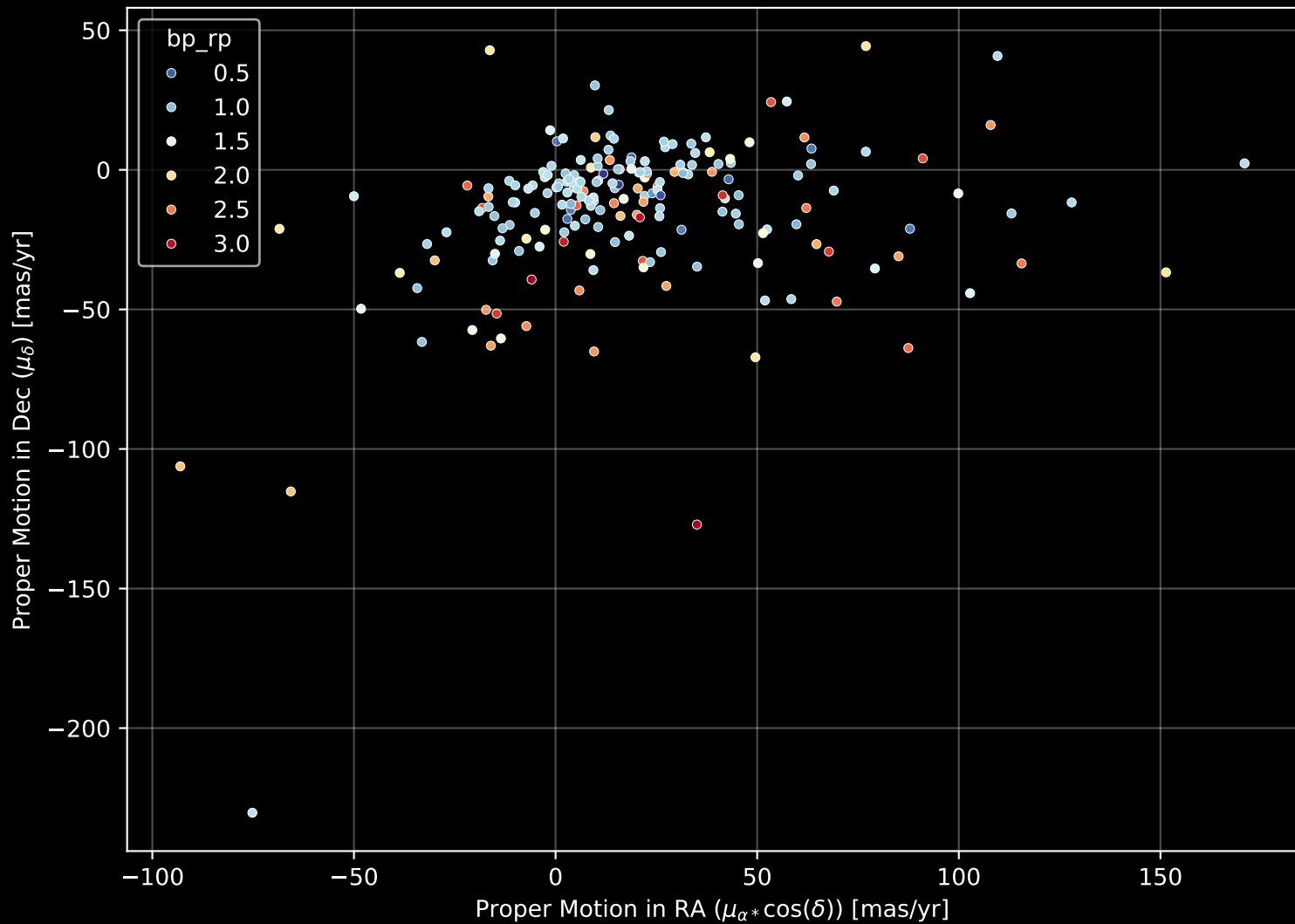
APOGEE DR17 Field: [K2_C8_129-62_btx] Proper Motion Diagram (n= 198)
