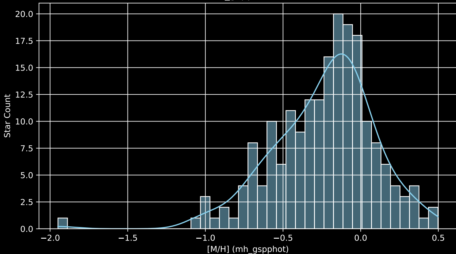
APOGEE DR17 Field: [K2_C8_129-62_btx [M/H] (mh_gspphot) (n= 196)
