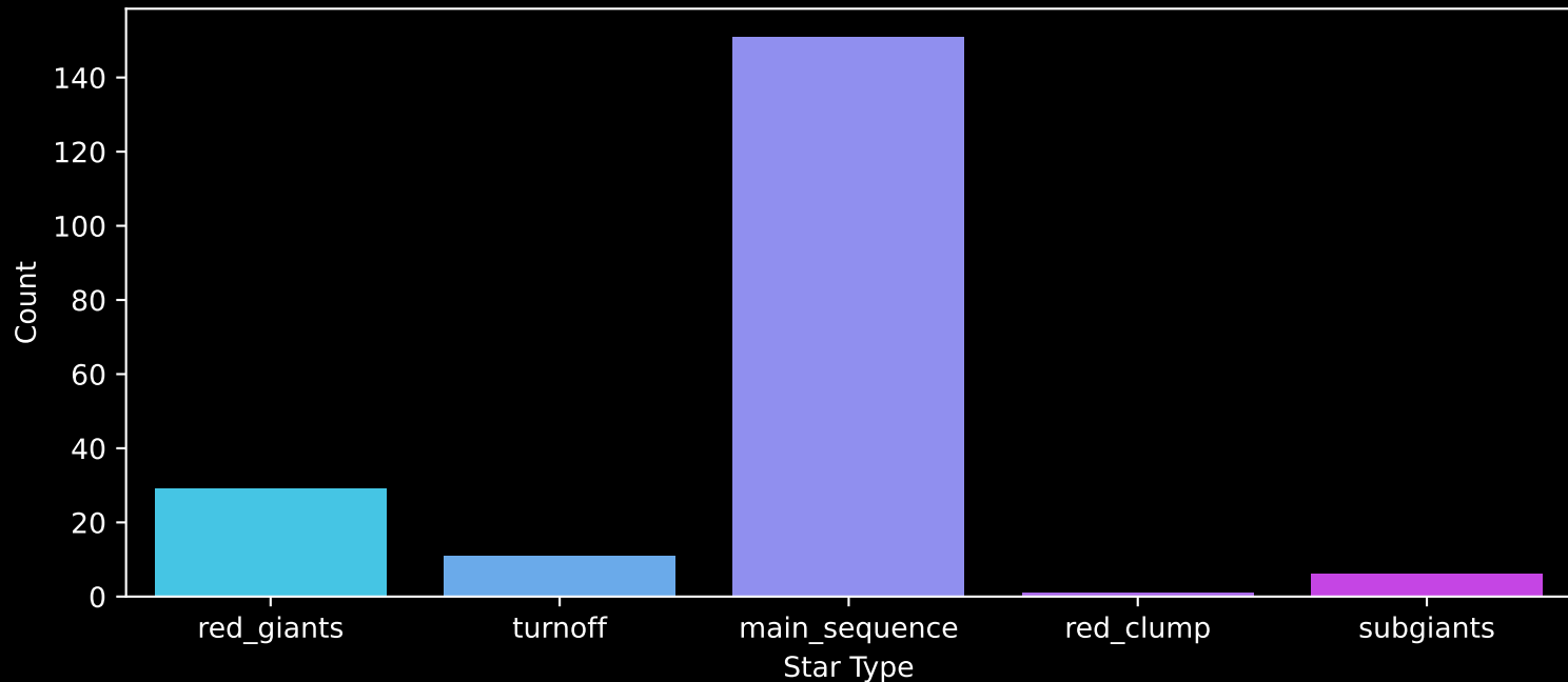
APOGEE DR17 Field: [K2_C8_129-62_btx] Count plot of Star Type
