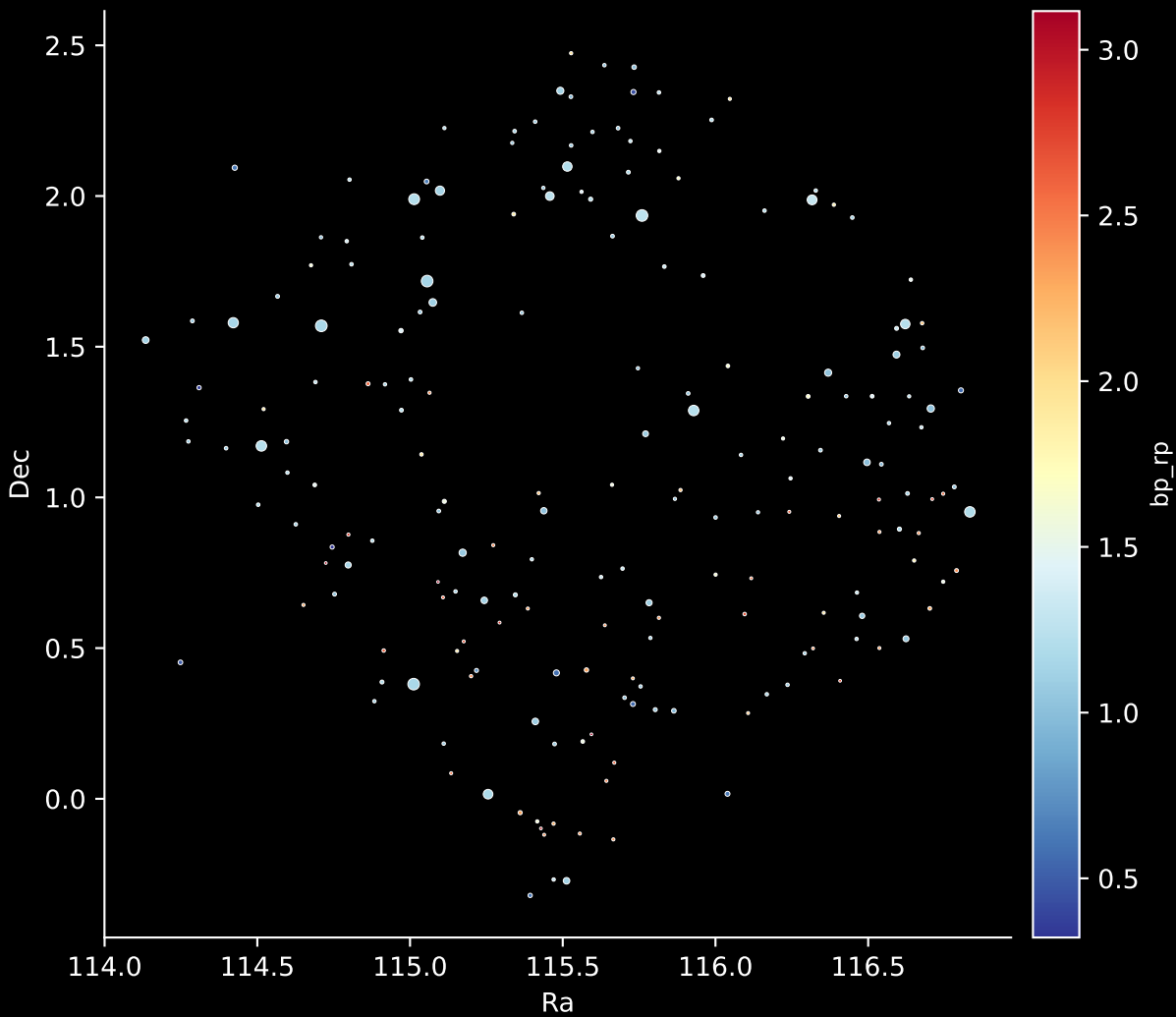
APOGEE DR17 Field: [K2_C8_129-62_btx] Stars: 198
