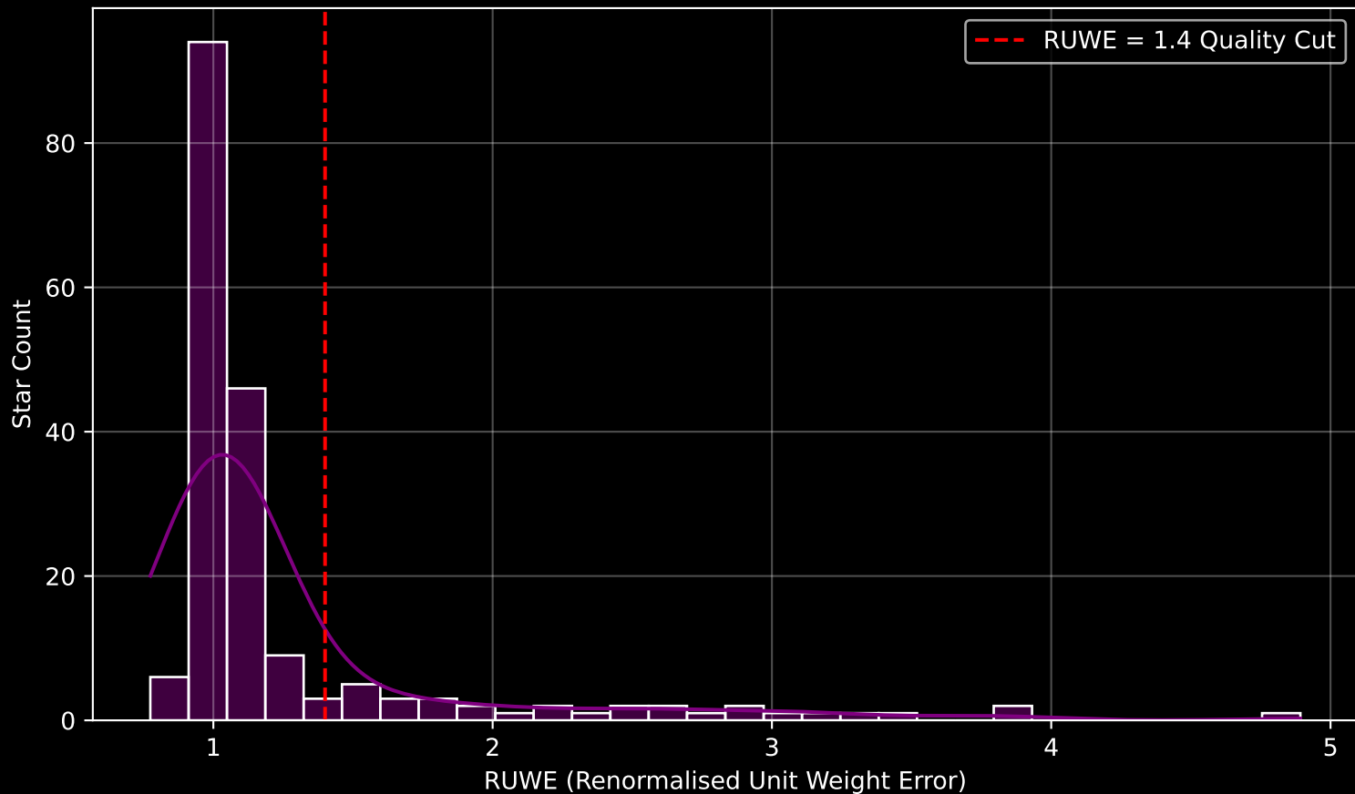
GAPOGEE DR17 Field [K2_C8_129-62_btx] RUWE Distribution (n= 189)
